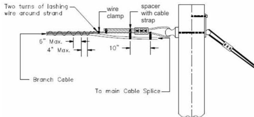
Figure 20– Pole Attachment at Dead-End Pole using Moving Reel Method (RUS 1751F-635)
