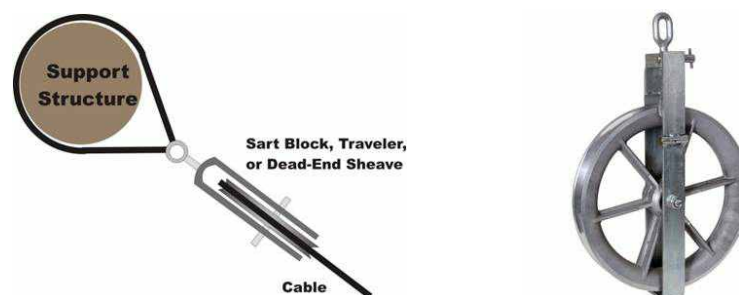
Figure 33- Supported Traveler or Large Diameter Sheave at Up-Feed and Down-Feed from Start and End Support Structures
