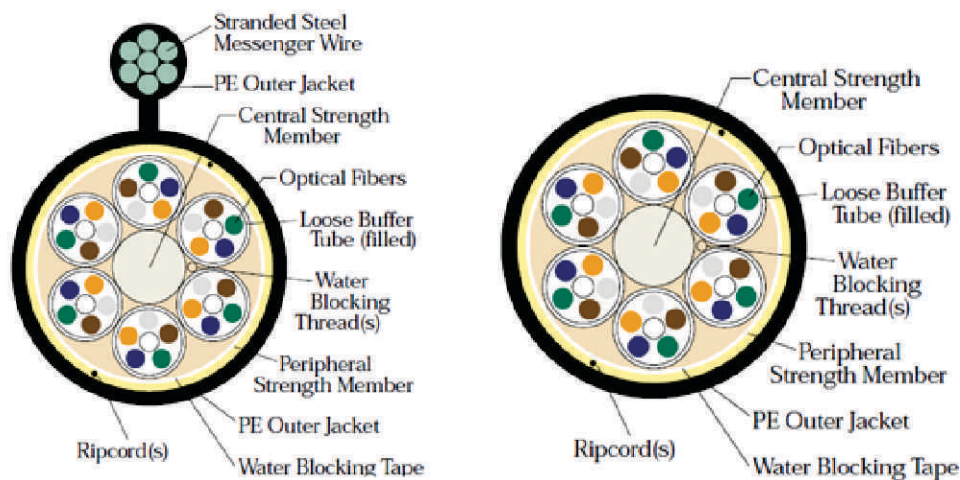
Figure 25– Two Main Self-Supporting Cables: Figure-Eight and ADSS Cables
