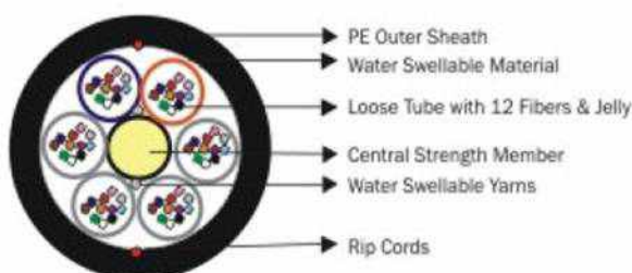
Figure 4– Cross-Section of Sterlite's Micro DUCT-LITE™ Multitube Fiber Optic Cable
