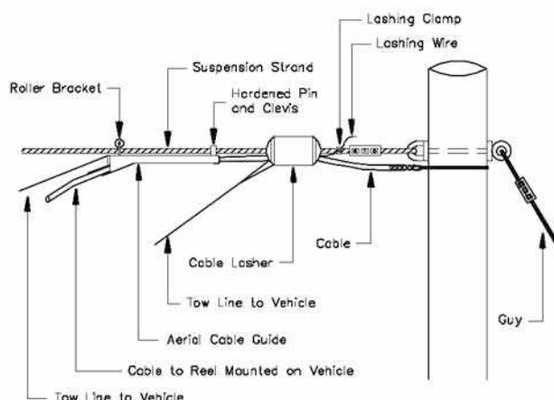
Figure 12– Start Up Configuration for Moving Reel Aerial Placement Method (RUS 1751F-635)
