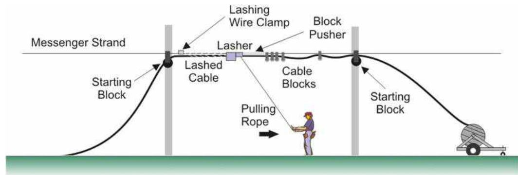
Figure 19– Stationary Reel Method Lashing Aerial Cable to Messenger Strand Being Pulled in the Opposite Direction of the Cable Placing Operation
