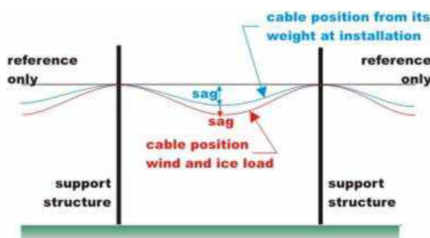
Figure 6– Sag Drawing of Aerial Plant Catenary Cable Deflection
