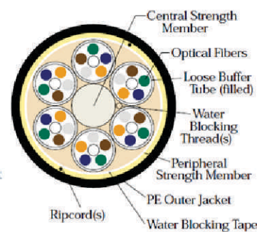
Figure 1– Sterlite Duct-Lite™ Optical Cable for Lashed Aerial Applications
