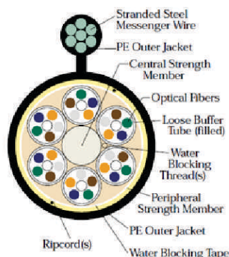
Figure 2– Sterlite Loose Tube Figure-Eight Optical Cable for Aerial Applications
