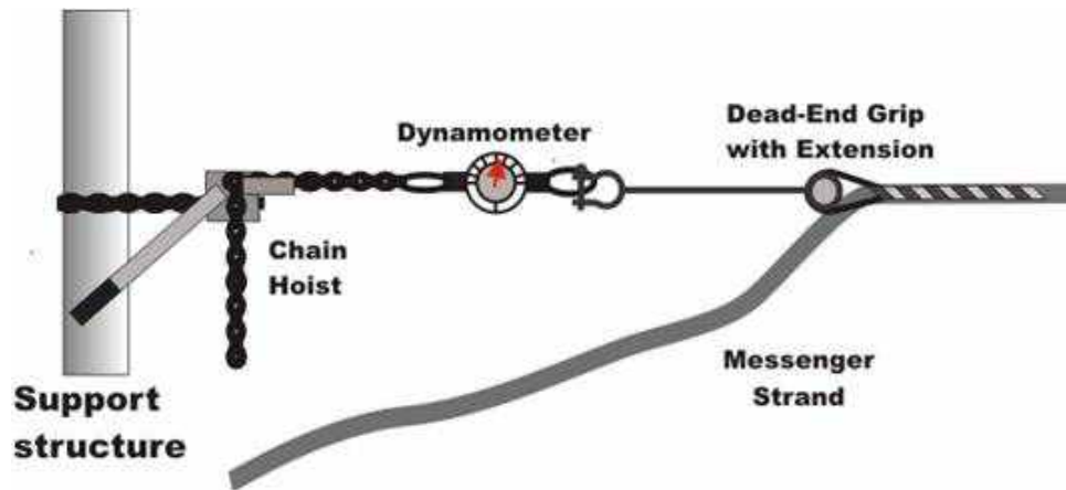
Figure 7– Tensioning the Messenger Strand Using a Dynamometer and Chain Hoist
