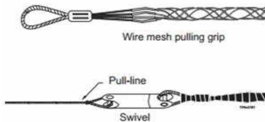
Figure 14– Pulling Hardware Required to Place Cable onto Cable Blocks During the First Stage of the Stationary Reel Placing Method
