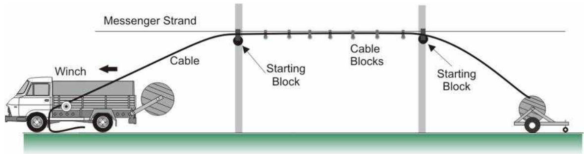
Figure 18– Stationary Reel Method, Cable Being Pulled into Cable Blocks Prior to Lashing Operation
