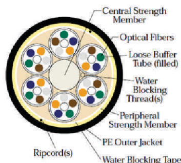
Figure 3– Sterlite Aerial-Lite™ (ADSS) Optical Cable for Aerial Applications
