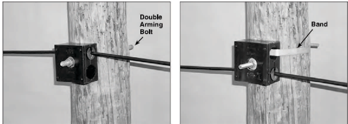
Figure 40– FIBERLIGN® Lite Tangent Supports Bolt-Mounted (Left) and Band-Mounted (Right).
